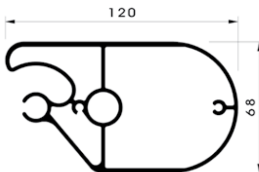
VARISOL W500 Fallstange
