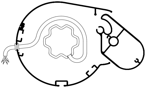
VARISOL W500 Standard-Kabelabgang
