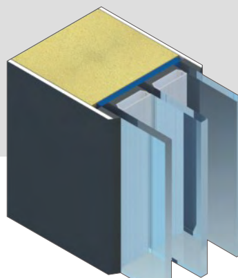
Panel ISOGLAS U_g = 0,5 \text{ W/m}^2\text{K}
